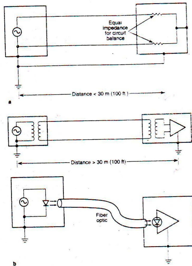
FIG. 6.22 Eliminating ground noise. Circuit balance or isolation removes problems from ground noise. (a) For short distances, a balanced transmission line and single-point grounding reduce noise and safety concerns. (b) For long distances, an isolated signal transmission allows multiple safety grounds while eliminating ground loops.
