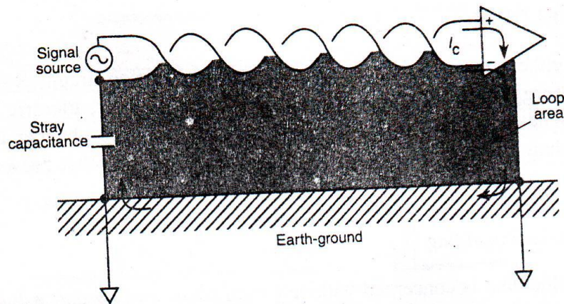
FIG. 6.33 Twisted-pair cable. Twisting the wire and running it close to the ground will reduce the common-mode current, I_c , by reducing the loop area for inductive coupling .
