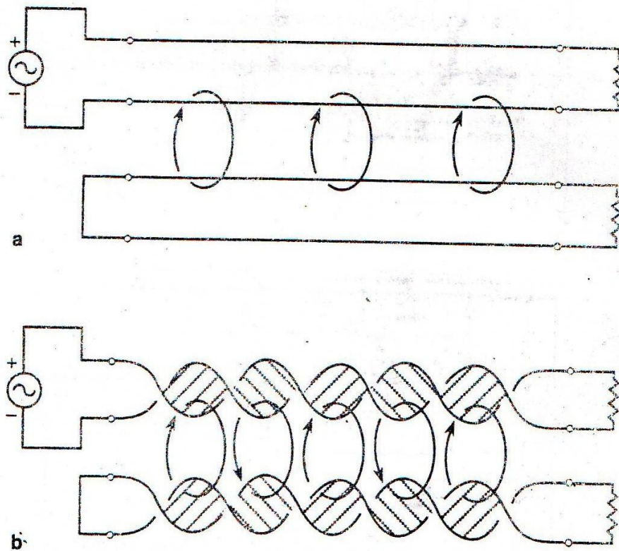
FIG. 6.14 Effect of twisted wire. (a) Straight wires create small loops that can couple magnetically. (b) Twisted wire eliminates the effective loop area of cables and magnetic coupling.
