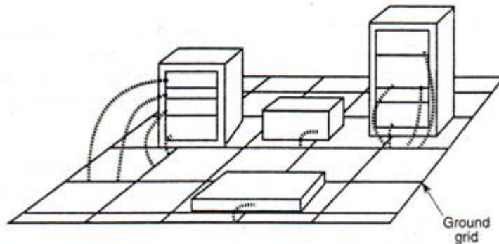
FIG. 6.20 A ground grid. Such grounding is appropriate for high-frequency operation or high-fault currents.
