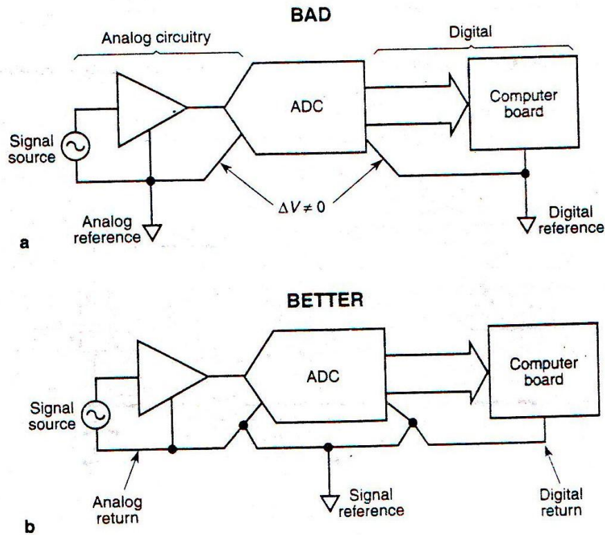
FIG. 6.19 Reducing noise from the signal reference. Tie the analog and digital references together near the ADC. (a) Separate references can lead to large loops of current. (b) A single-point reference eliminates large loops; usually an uninterrupted ground plane suffices.
