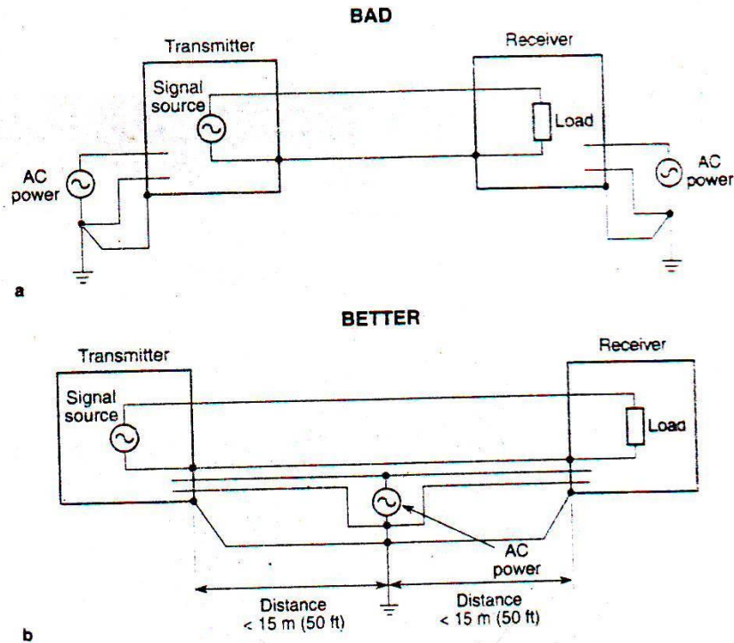
FIG. 6.23 Coordinated routing of power, signal, and safety ground. (a) Separate grounds and power, while safe, introduce noise. (b) For short distances, a coordinated routing of power and ground maintains safety and reduces noise.
