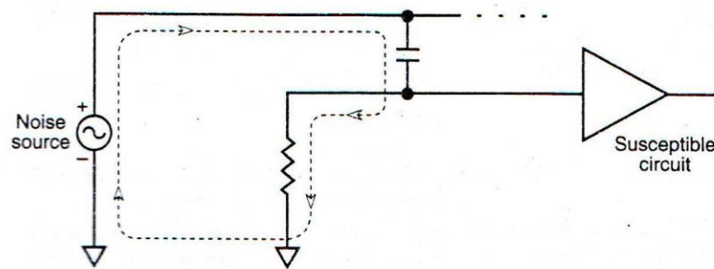
FIG. 6.7 Capacitive coupling. Coupling from stray capacitance completes the circuit of a noise source into a susceptible circuit.
