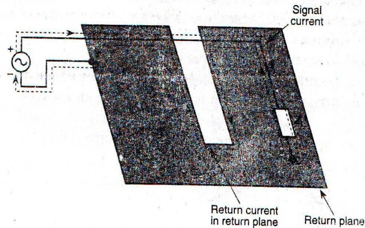
FIG. 6.13 A slot in the return plane increases the current loop area and the self-inductance.
