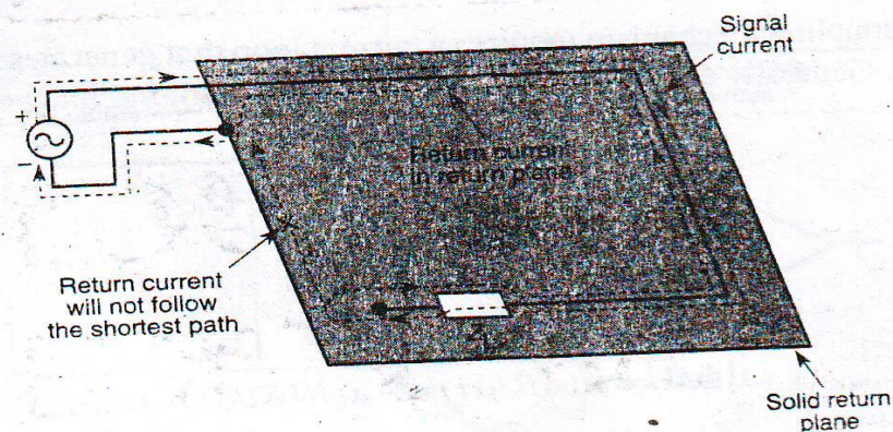
FIG. 6.12 Path of return current. Return current will follow the path of least impedance (in this case, the least self-inductance), not necessarily lowest resistance.
