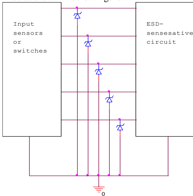
Fig: Preventing damage by shunting high voltage transients away from circuits with zener diodes or MOVs
