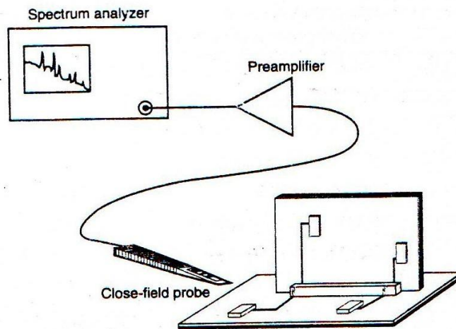
FIG. 6.45 Use of close-field probe to detect individual components, circuits, or shields that are radiating EMI.
