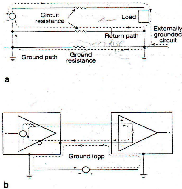
FIG. 6.10 A ground loop. Multiple ground connections can provide multiple return paths that cause significant current flow in the grounding structure, as shown in part (a). Ground potential causes currents in ground loops that unbalance circuits, as shown in part (b).
