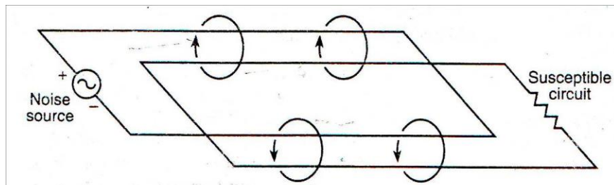
FIG. 6.6 Inductive coupling. Magnetic flux couples energy from the circuit of the noise source to the susceptible circuit.
