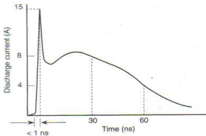
Fig: Discharge waveform at 4 kv
