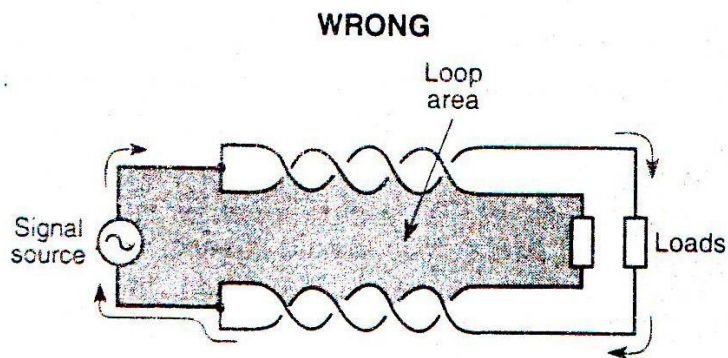
FIG. 6.32 Incorrect application of twisted-pair wire. A large loop area still exists.
