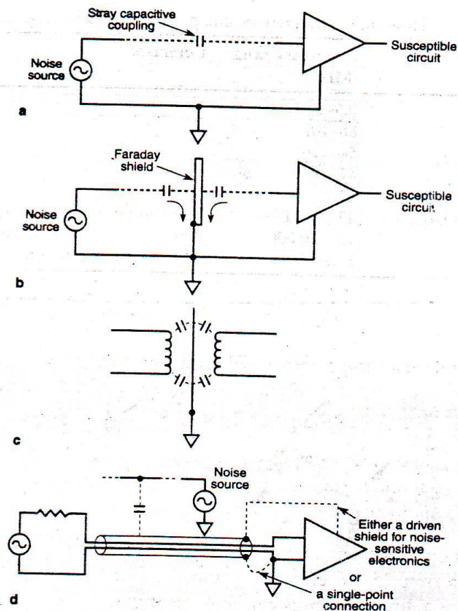
FIG. 6.34 Capacitive shielding. Capacitive coupling provides a path for the injection of noise charges, while an appropriately placed shield prevents the coupling between circuits by shunting charge to ground. (a) Outline of capacitive coupling. (b) Proper placement of a shield to shunt noise charge. (c) A shielded transformer prevents capacitive coupling between windings. (d) A cable shield usually should be connected at only one place to prevent coupling or shunt charge.
