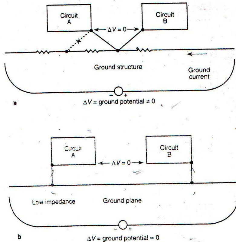
FIG. 6.16 Two grounding configurations. [For safety and for signal reference, reduce the potential difference between the ground connections of circuit, instrument, or chassis] (a) Single-point ground . (b) Multipoint ground with low-impedance ground structure .
