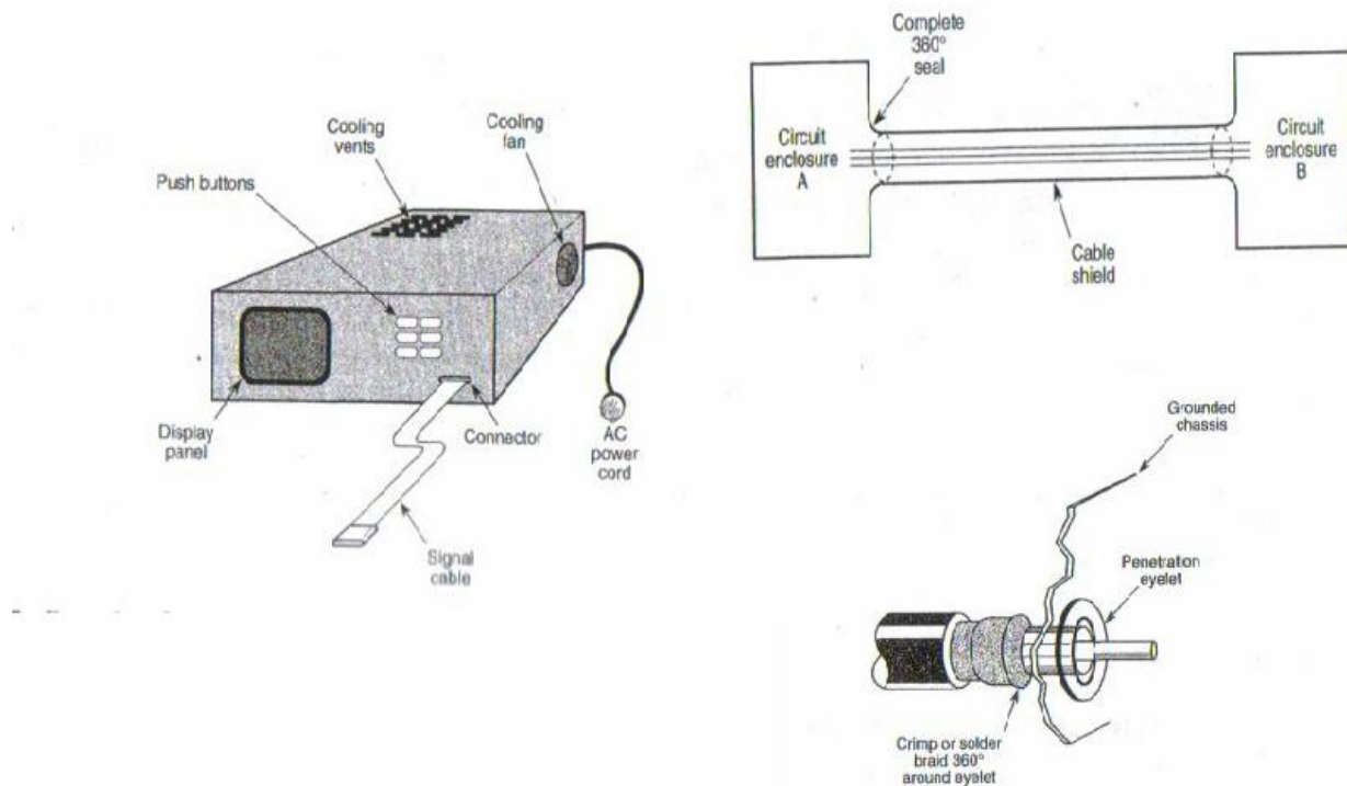
Fig: Shielded enclosure and cable shield
