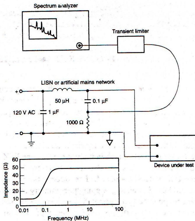
FIG. 6.46 Measuring conducted EMI by powering the device under test through a line impedance stabilization network (LISN): The LISN, or artificial mains network, isolates the test circuit from emissions conducted from the input power mains. The transient limiter presents damage to the spectrum analyzer when the LISN is switched into use.
