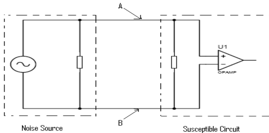
Fig: Conductive coupling. If either connection A or B is removed, the conductive noise is eliminated.
