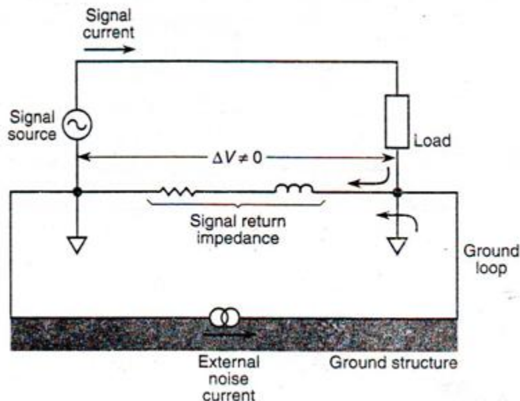
FIG. 6.21 A ground loop. It occurs when a circuit makes multiple connections to the ground conductor or structure.
