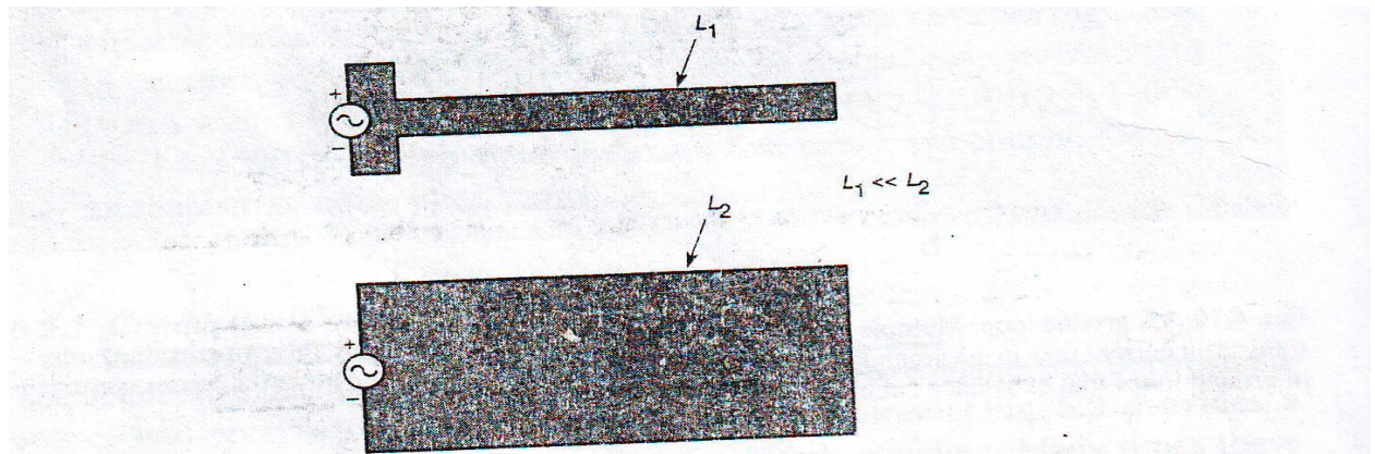
FIG. 6.11 Reducing loop area. Small loops of current have lower self-inductance and thus lower impedance.
