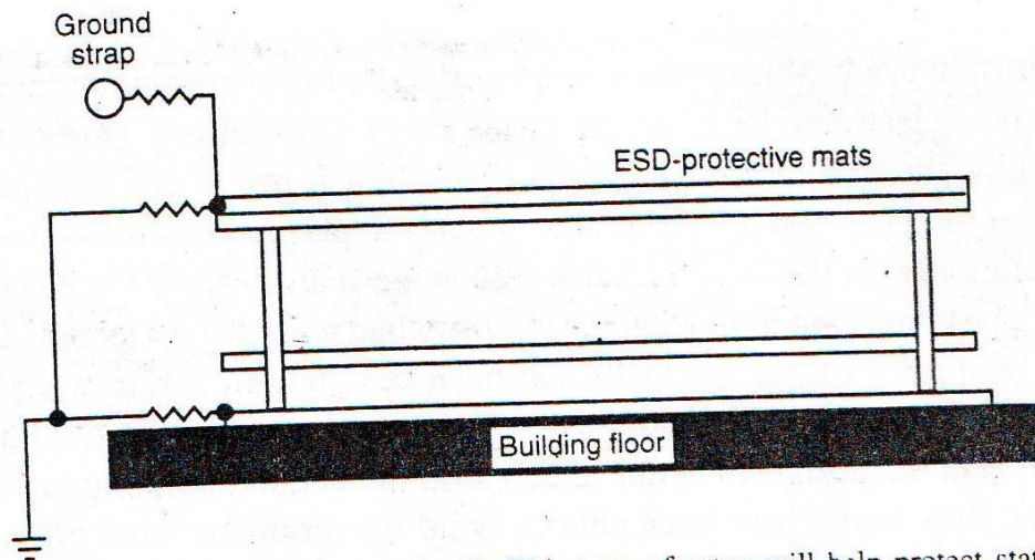
FIG. 6.43 Typical ESD-grounded workbench. This type of setup will help protect static-sensitive components.
