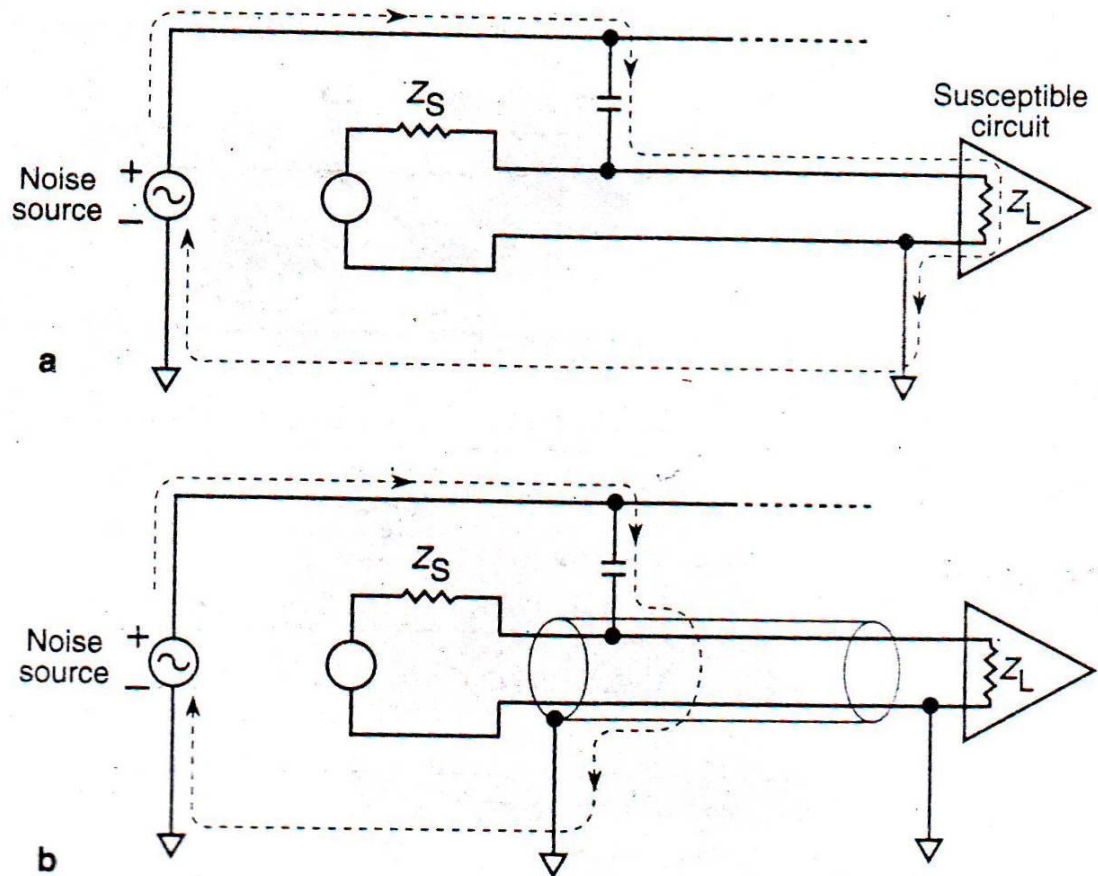
FIG. 6.15 Effect of shielding. (a) Without the shield, stray currents can disrupt susceptible circuits. (b) A properly connected shield can divert capacitively coupled current from susceptible circuits.
